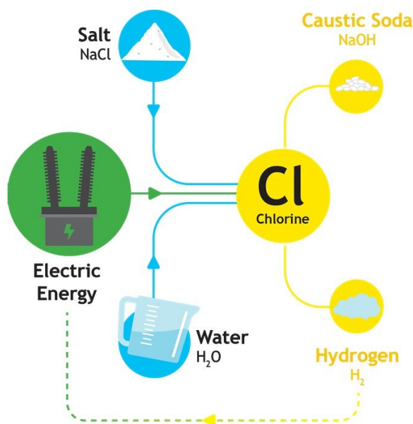
Figure 1. The chlor-alkali production process
